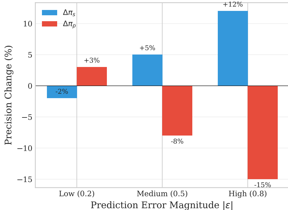
(b) Precision Response to Error
