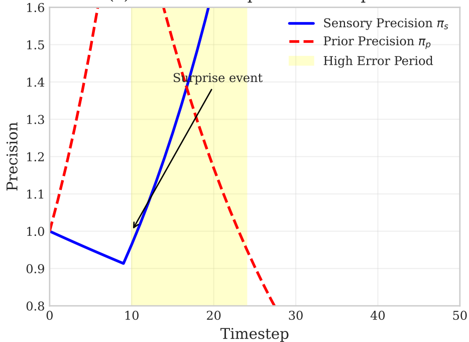
(a) Precision Adaptation to Surprise
