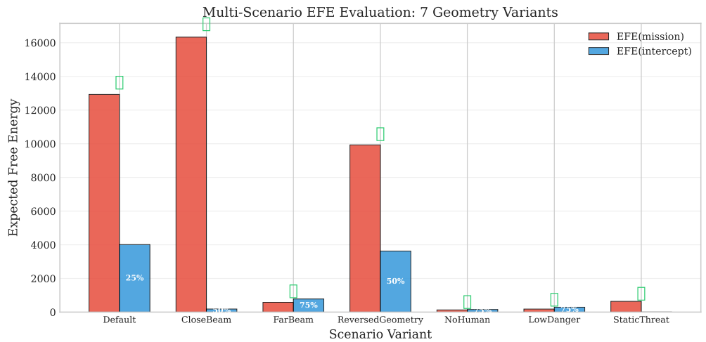
Figure 8. Multi-scenario EFE evaluation. Checkmarks indicate correct decisions. The agent intercepts when safety EFE dominates (Default, CloseBeam, Reversed, StaticThreat) and continues the mission otherwise (FarBeam, NoHuman, LowDanger).
