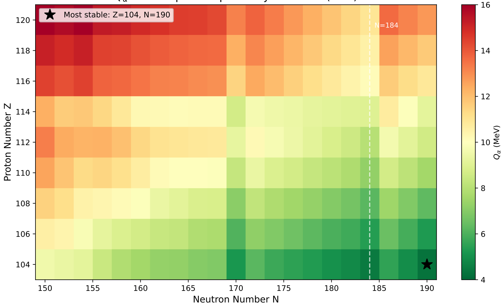
Q_\alpha Landscape of Superheavy Elements (MeV)
