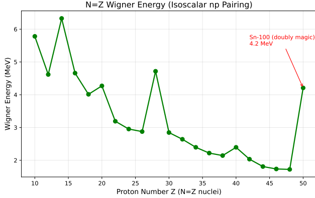
Figure 4: N = Z Wigner energy. The non-monotonic enhancement at Z = 50 (Sn-100) reflects constructive interference of isoscalar pairing with shell closure [9].
