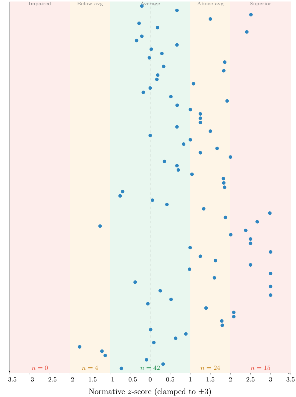
Figure 8: Forest plot of normative z-scores for 85 benchmarks with matched human baselines (z-scores clamped to \pm 3 for readability). Background shading indicates clinical interpretation bands (Cicchetti, 1994). Band counts: 42 Average ( |z| \leq 1 ), 24 Above Average, 4 Below Average, 15 Superior ( z > 2 ), 0 Impaired ( z < -2 ). Data loaded from normative_zscores.csv .
