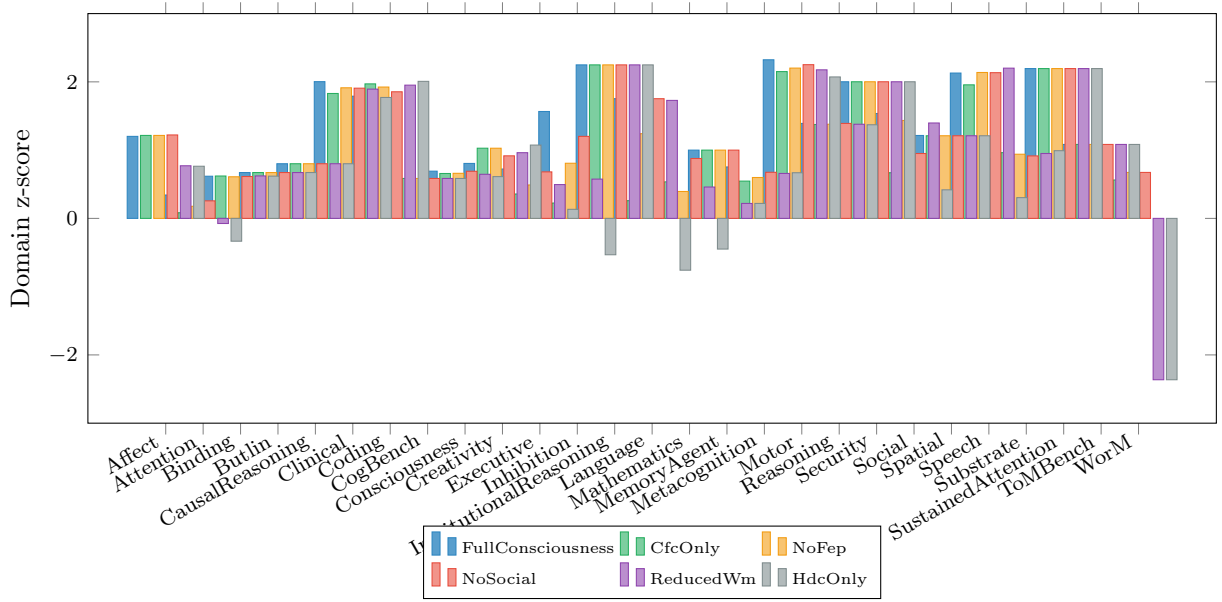
Figure 9: Ablation comparison across six presets and 27 cognitive domains. HDCOnly (Cohen’s d = 0.64 ) produces the largest overall deficit, with WorM ( \Delta = 3.09 ), Language ( \Delta = 2.51 ), and Inhibition ( \Delta = 2.10 ) most affected. ReducedWM selectively devastates WorM ( \Delta = 3.09 ) while leaving other domains largely intact. Several domains ( InstitutionalReasoning , CausalReasoning , Security , SustainedAttention , ToMBench ) are ablation-invariant ( \eta^2 = 0.000 ), reflecting reliance on structural HDC operations unaffected by encoding noise. Data loaded from ablation_domains.csv .
