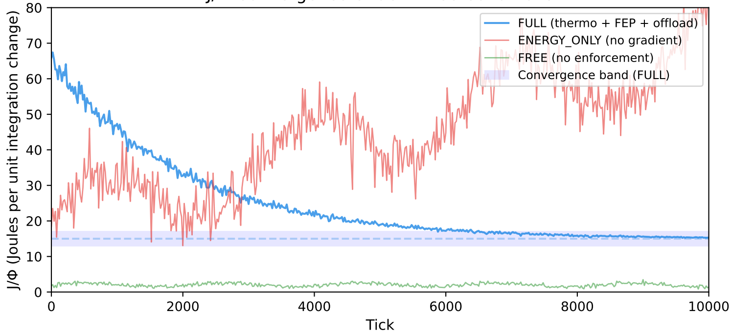
J/ \Phi Convergence Under Three Conditions
