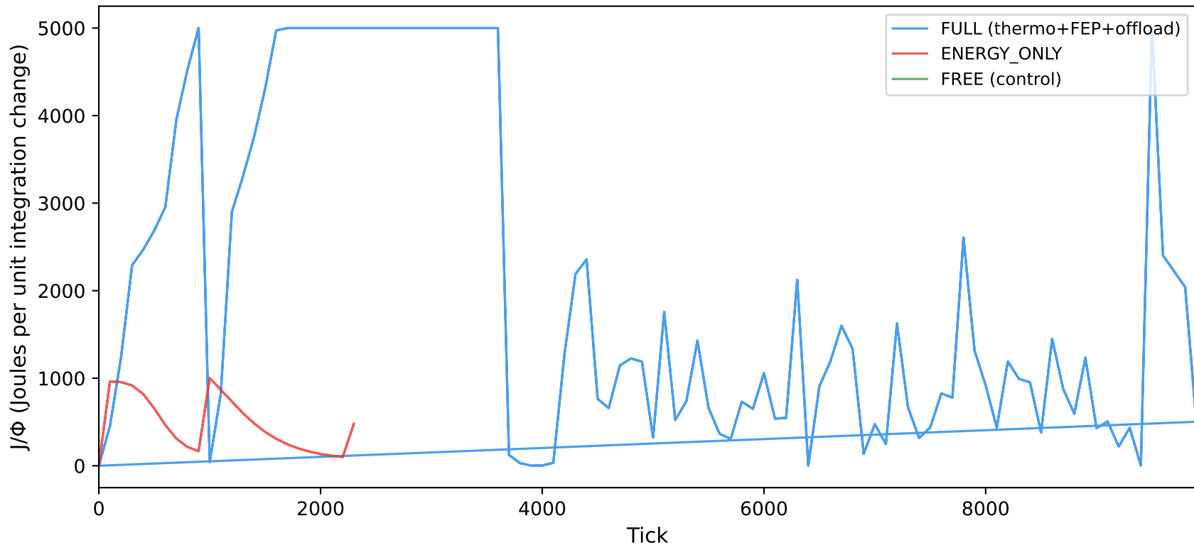
J/ \Phi Convergence — Real Simulation Data (seed=42)
