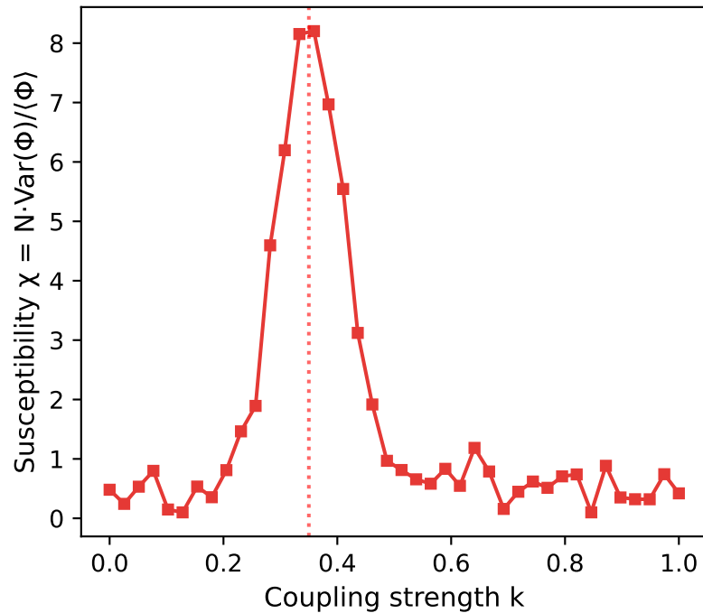
(b) Susceptibility (peaks at k_c )
