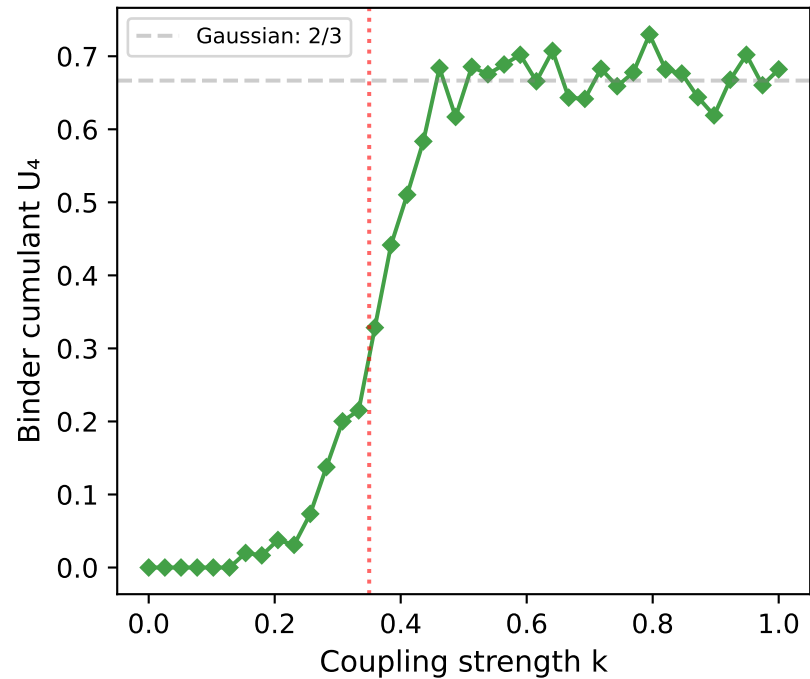
(c) Binder Cumulant
