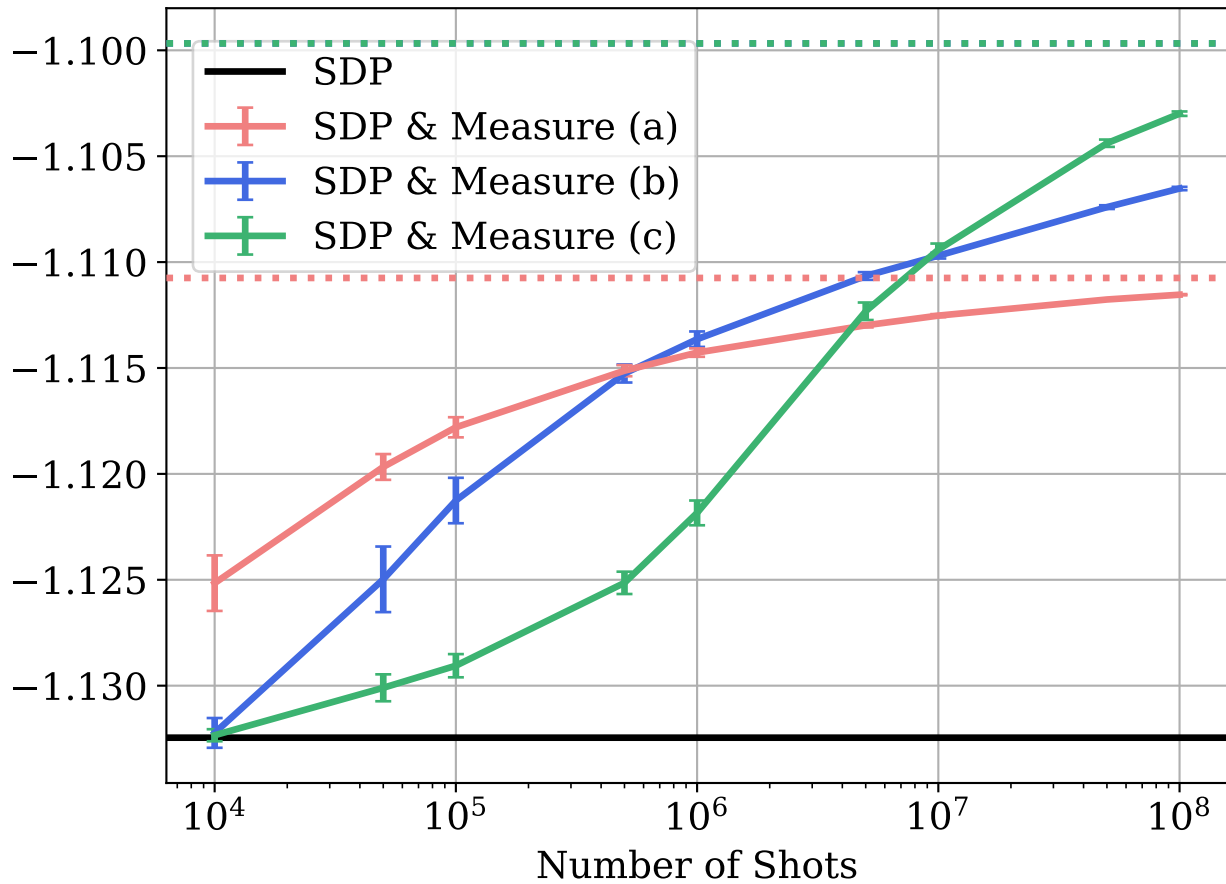
Ground-state Energy Lower Bound
