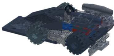
Brick-Composer
