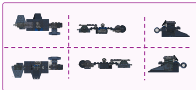
Brick-Composer
