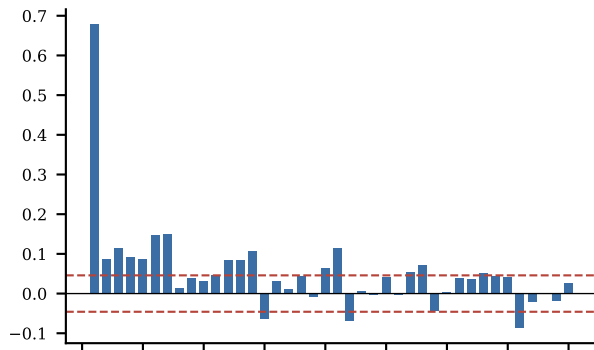
PACF (residual)
