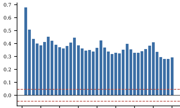
ACF (residual)
