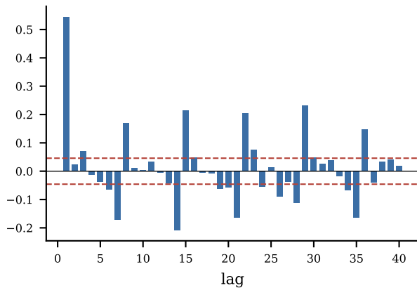
PACF (residual)
