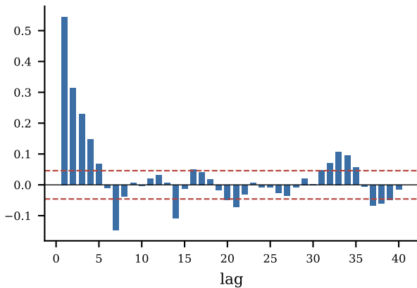
ACF (residual)
