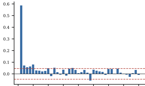
PACF (residual)
