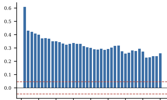
ACF (residual)
