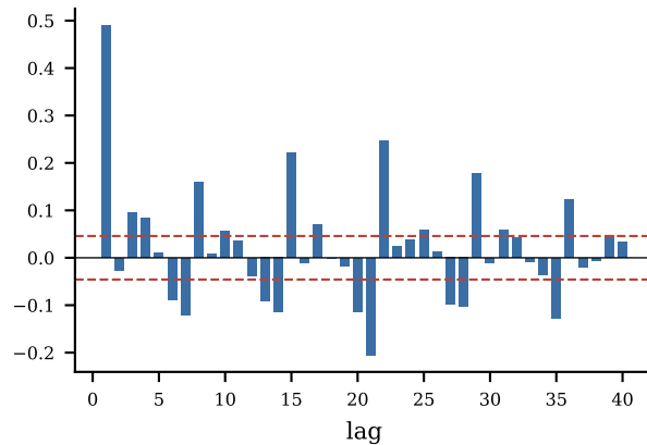
PACF (residual)
