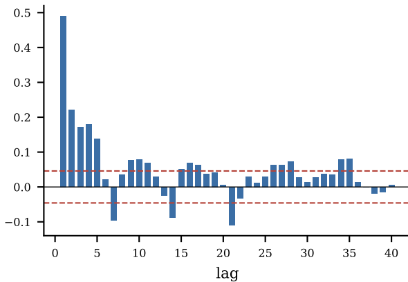
ACF (residual)
