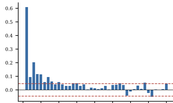
PACF (residual)
