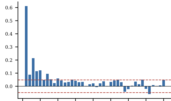
PACF (residual)
