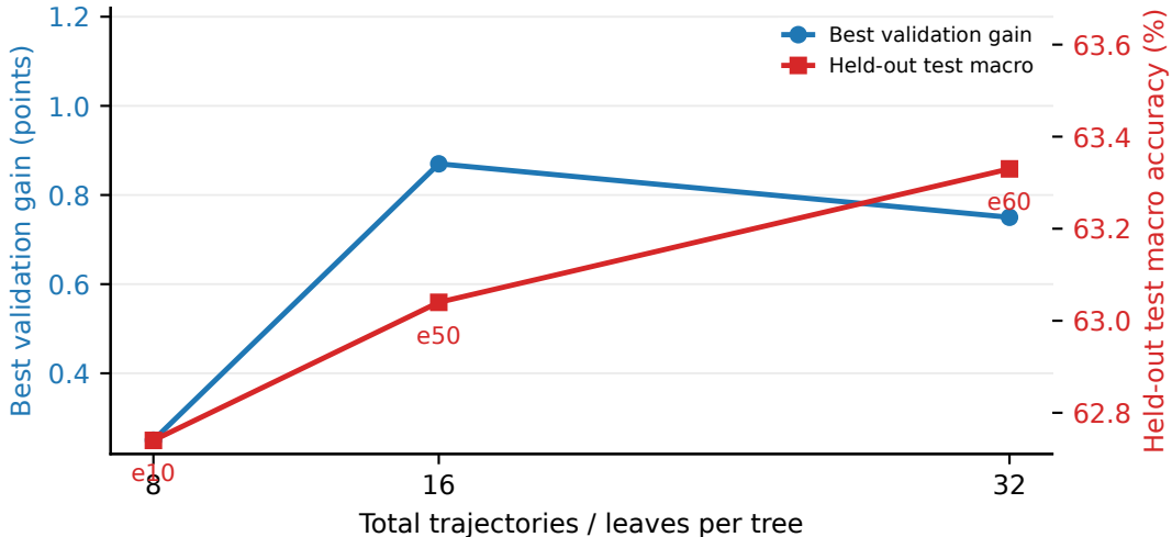
Qwen2.5-7B no-tool branch-budget sensitivity
