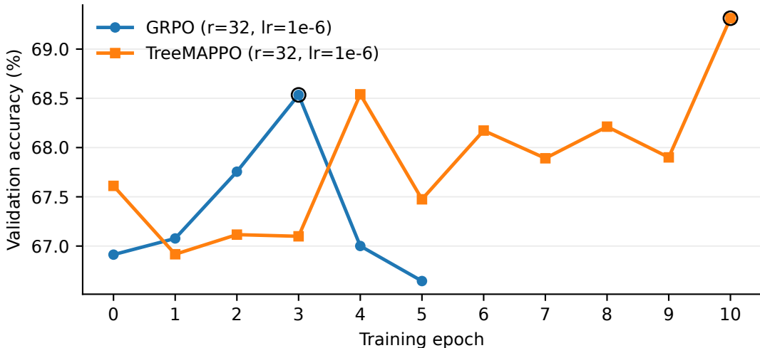
Qwen2.5-7B no-tool validation accuracy
