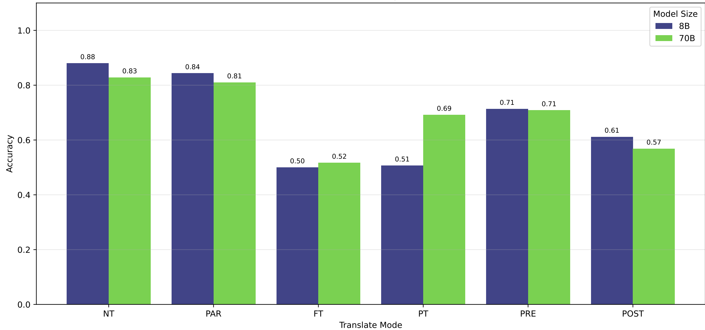
Llama-3.1 Model Size Comparison - Chinese
