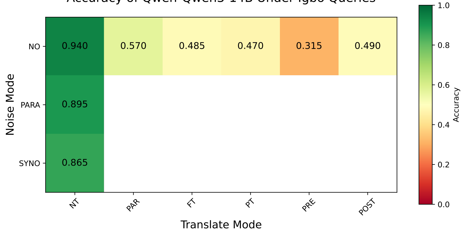
Accuracy of Qwen-Qwen3-14B Under Igbo Queries
