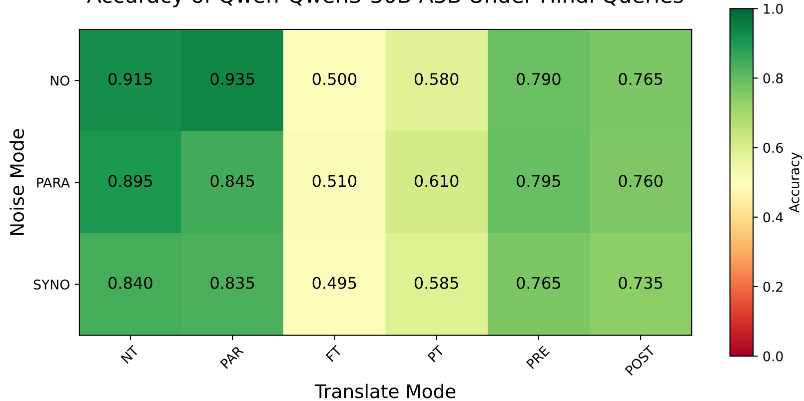
Accuracy of Qwen-Qwen3-30B-A3B Under Hindi Queries
