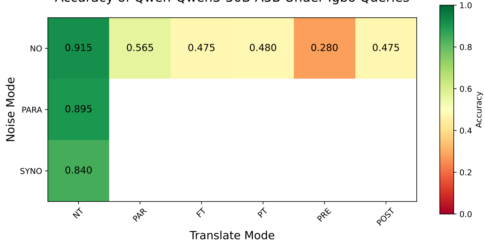
Accuracy of Qwen-Qwen3-30B-A3B Under Igbo Queries
