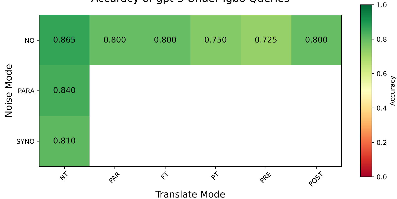
Accuracy of gpt-5 Under Igbo Queries
