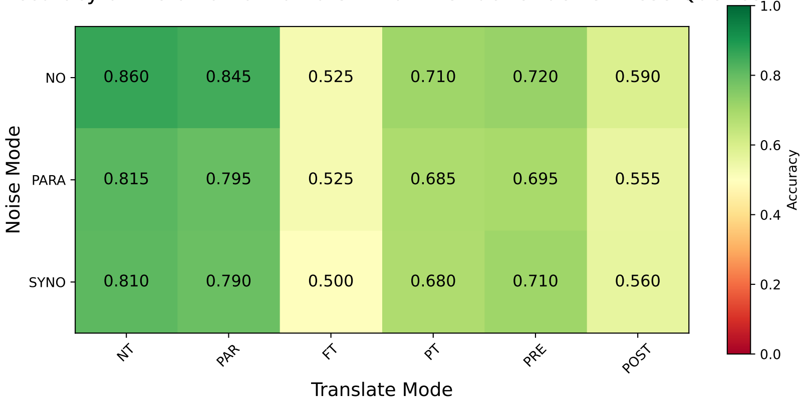
Accuracy of meta-llama-Llama-3.1-70B-Instruct Under Chinese Queries
