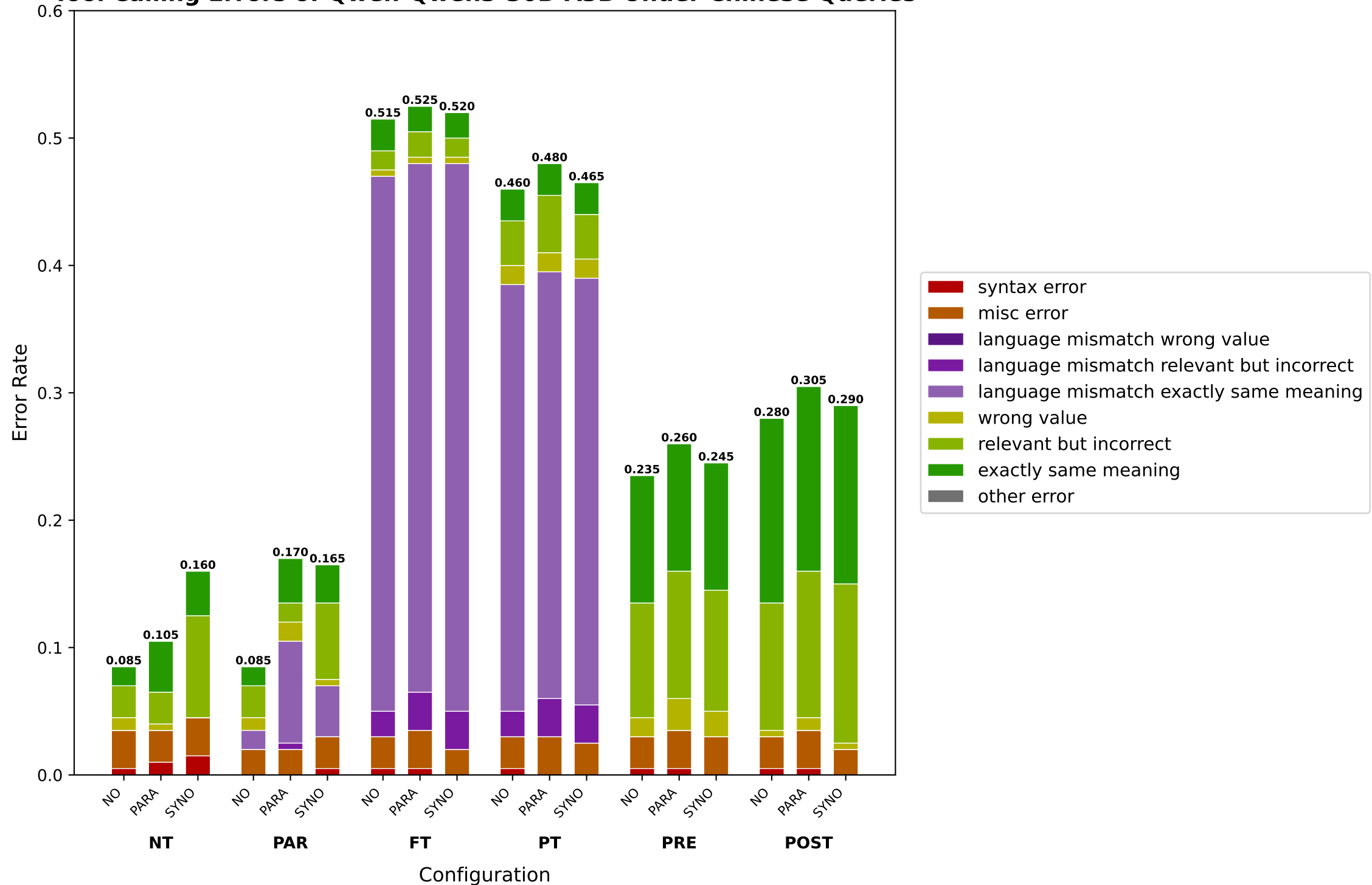
Tool Calling Errors of Qwen-Qwen3-30B-A3B Under Chinese Queries
