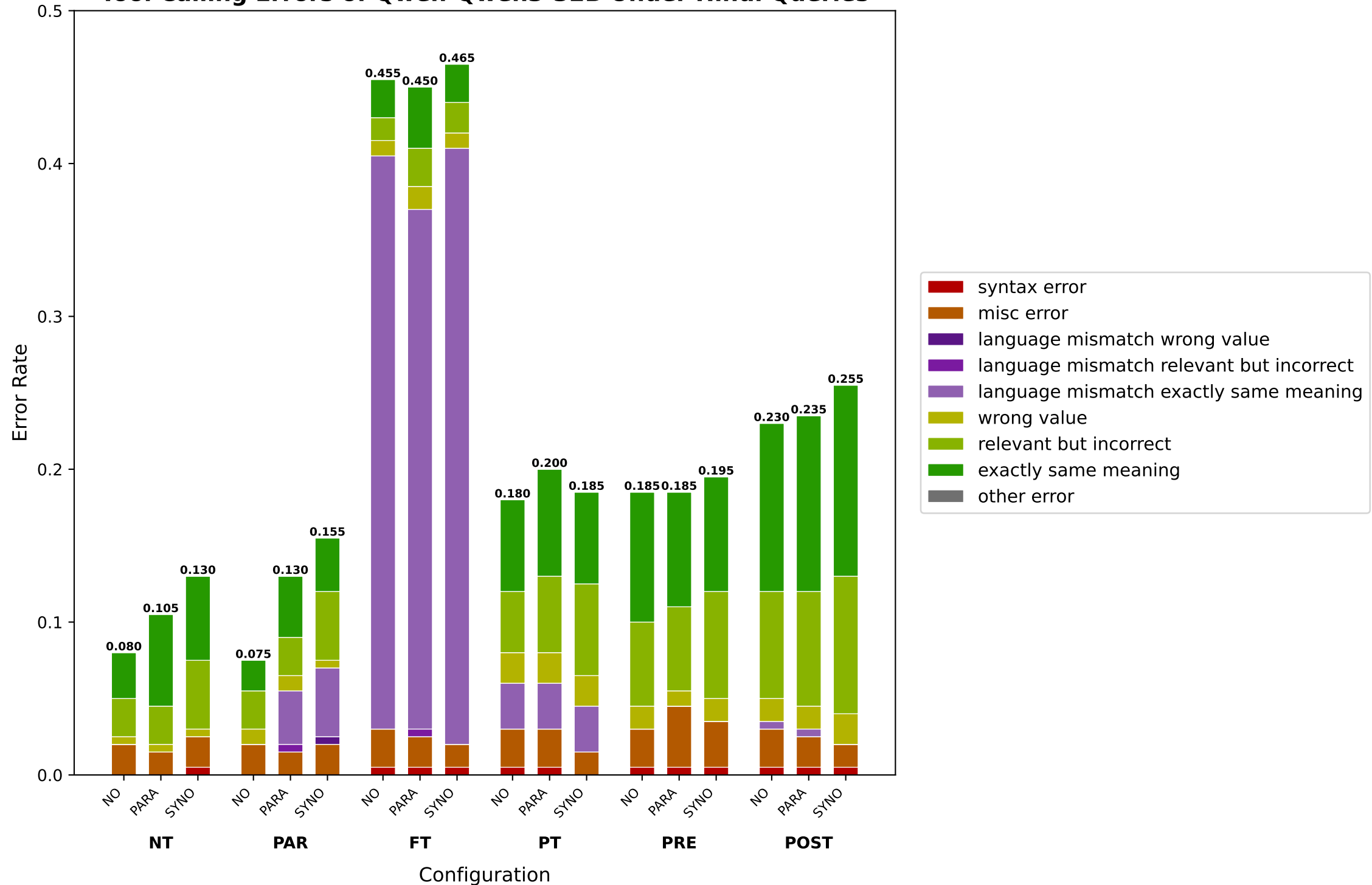
Tool Calling Errors of Qwen-Qwen3-32B Under Hindi Queries
