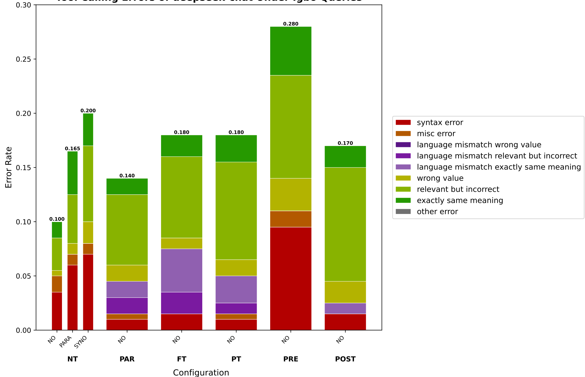
Tool Calling Errors of deepseek-chat Under Igbo Queries
