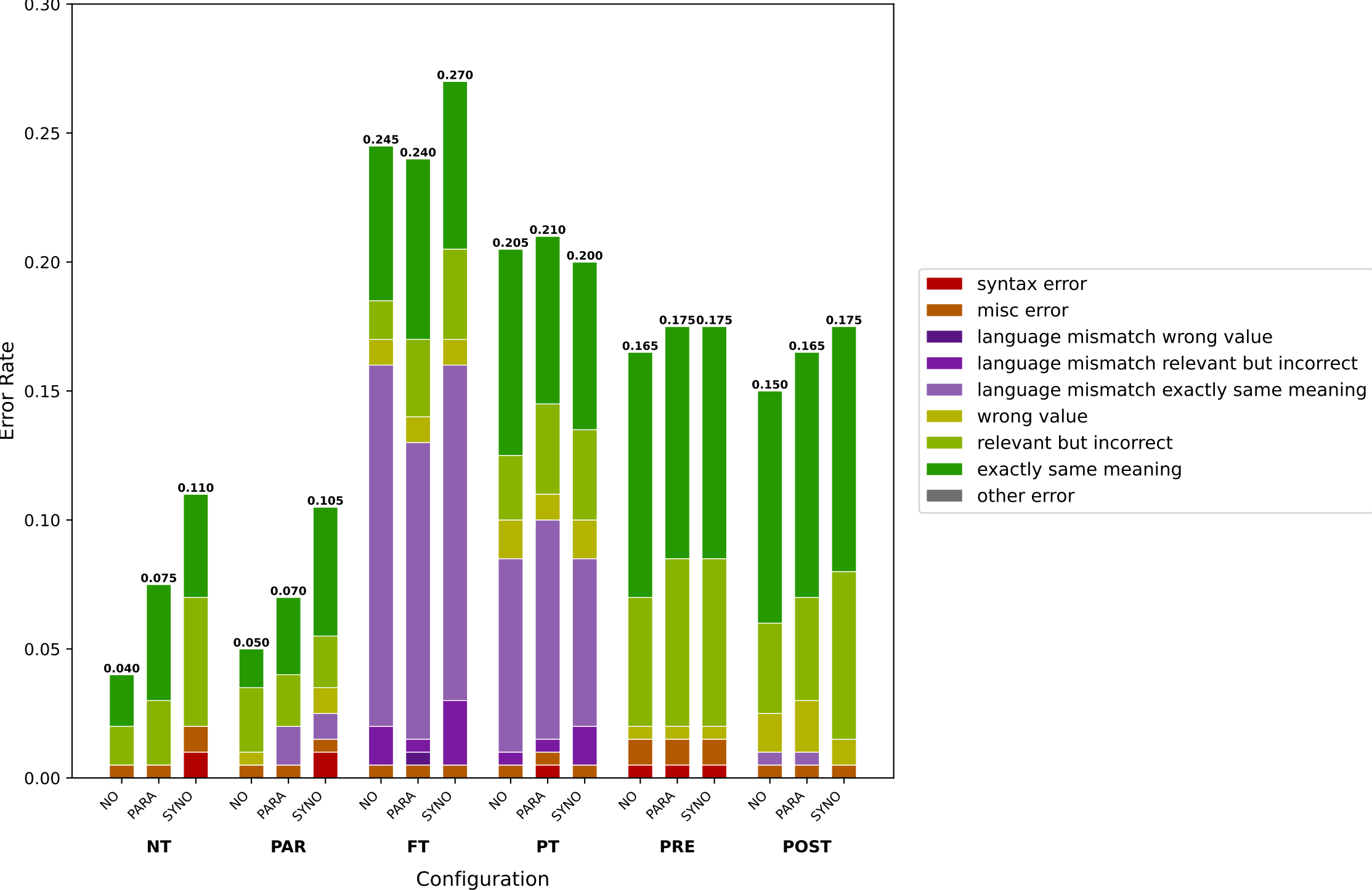
Tool Calling Errors of ibm-granite-granite-4.0-h-small Under Hindi Queries
