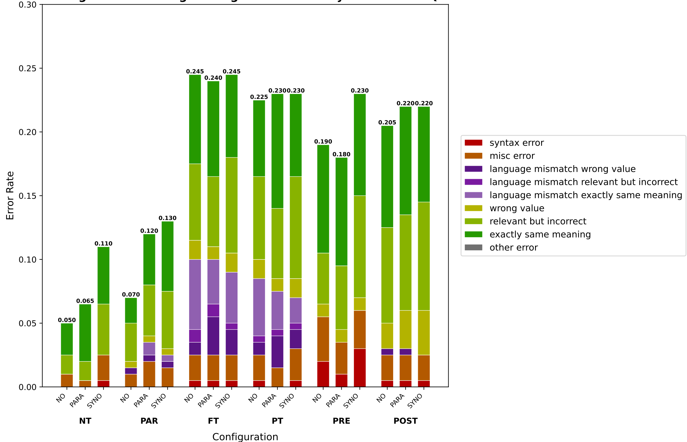
Tool Calling Errors of ibm-granite-granite-4.0-h-tiny Under Hindi Queries
