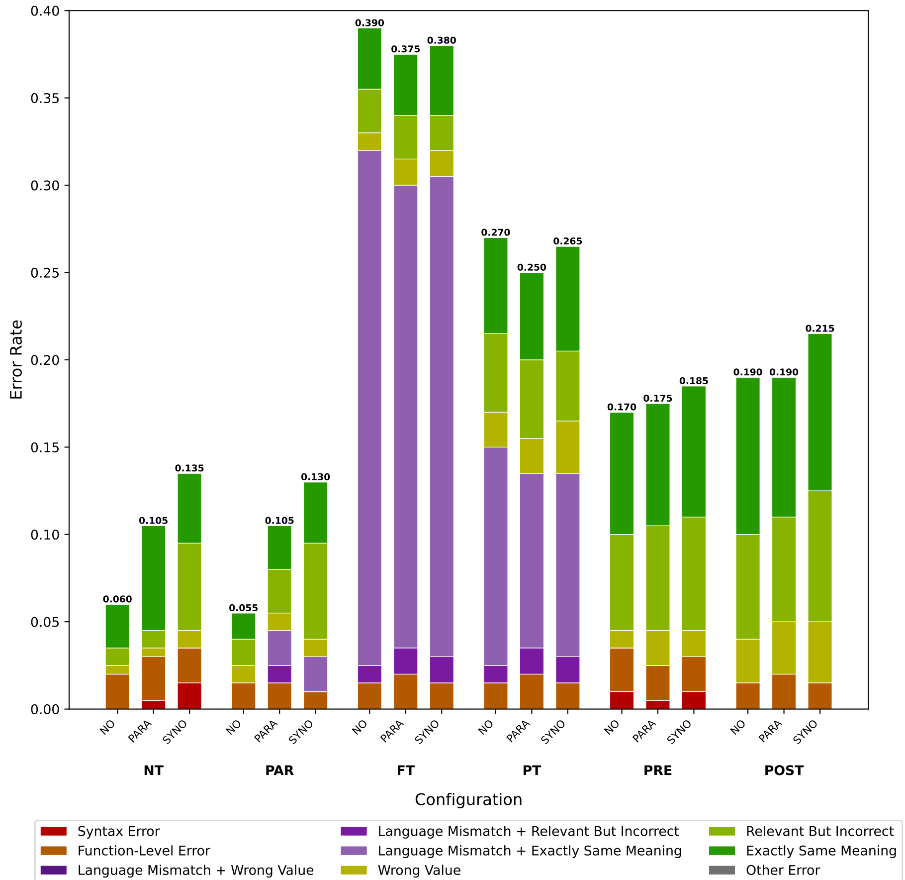
Tool Calling Errors of Qwen-Qwen3-14B Under Hindi Queries
