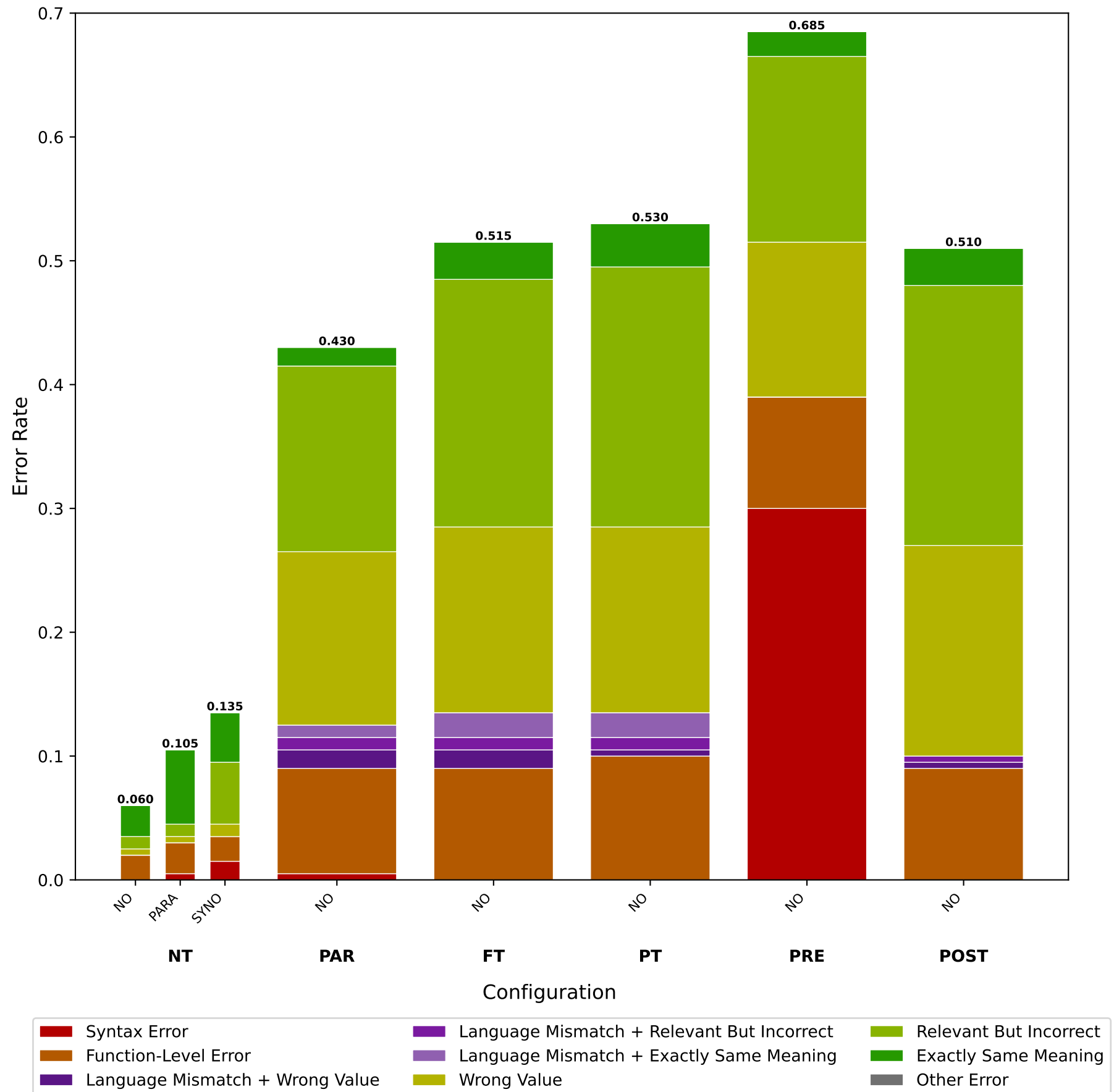
Tool Calling Errors of Qwen-Qwen3-14B Under Igbo Queries
