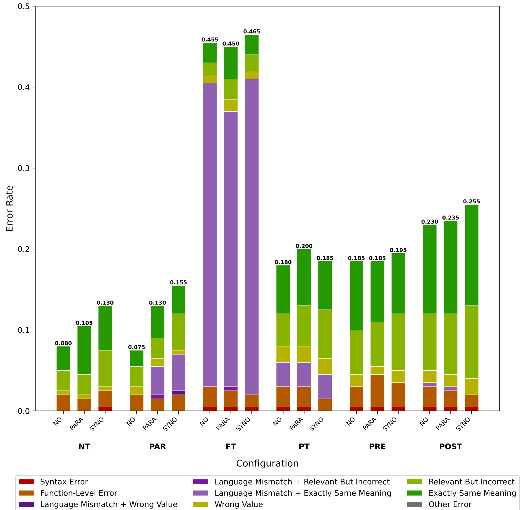
Tool Calling Errors of Qwen-Qwen3-32B Under Hindi Queries
