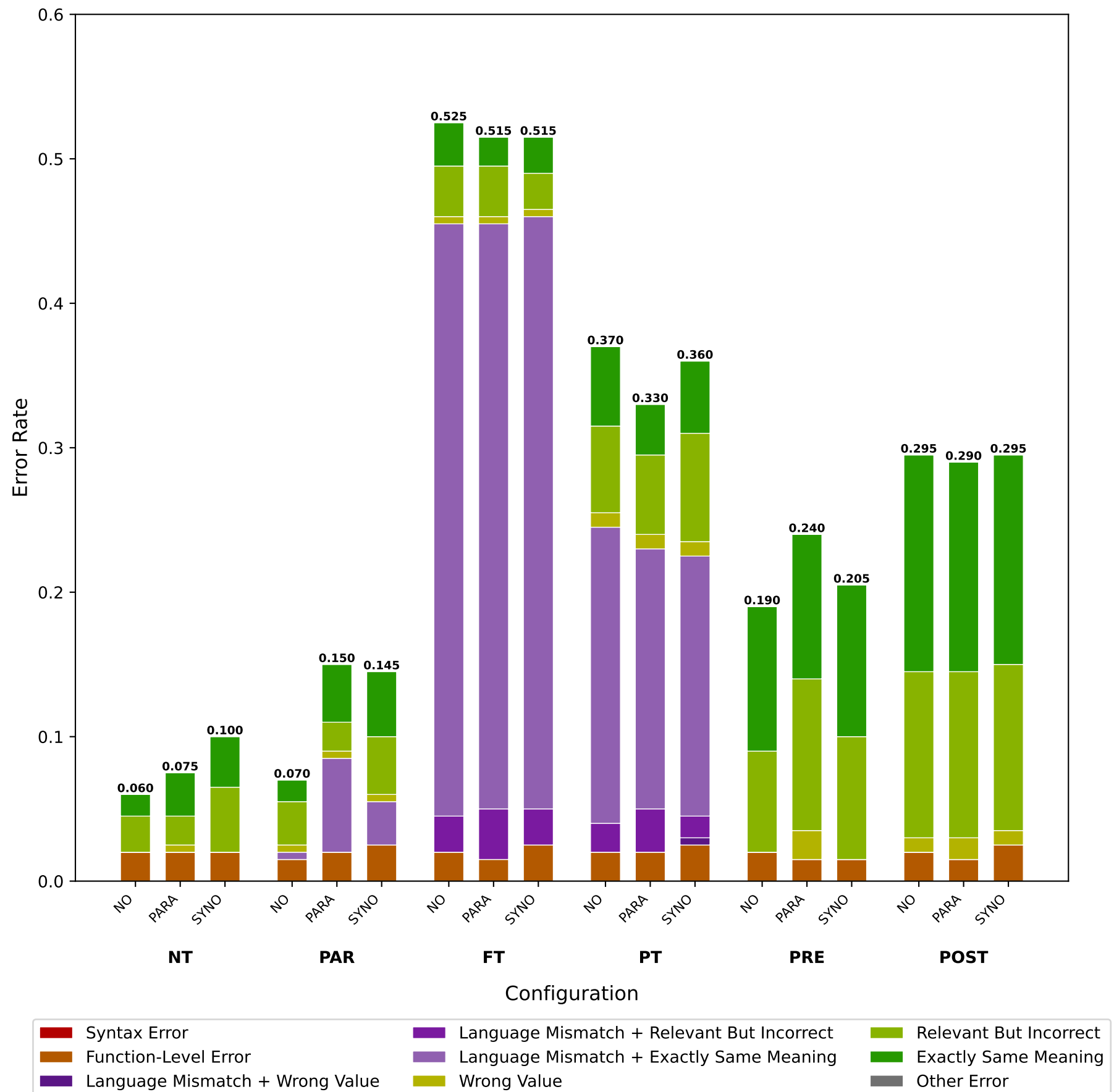
Tool Calling Errors of Qwen-Qwen3-8B Under Chinese Queries
