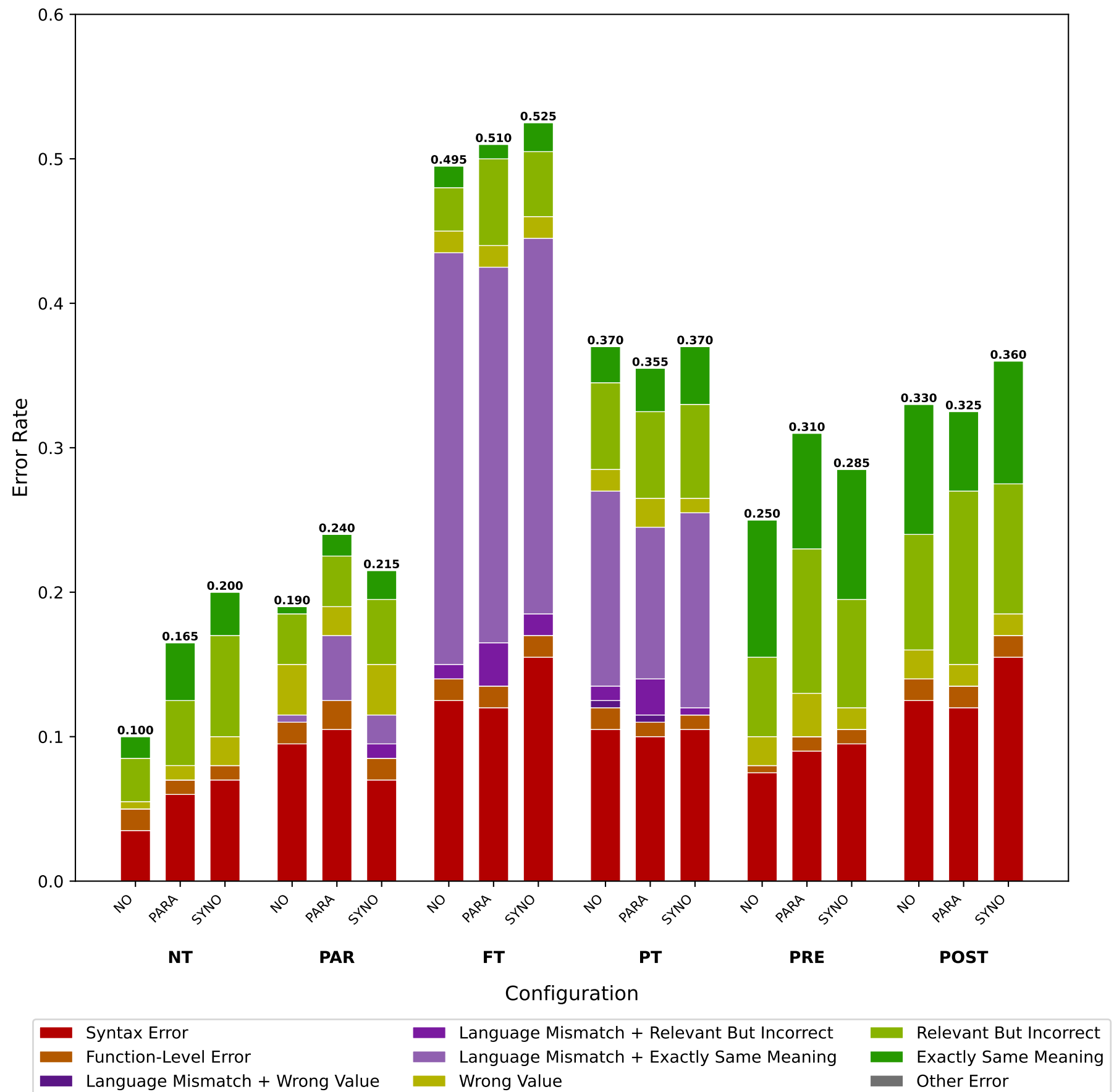
Tool Calling Errors of deepseek-chat Under Chinese Queries
