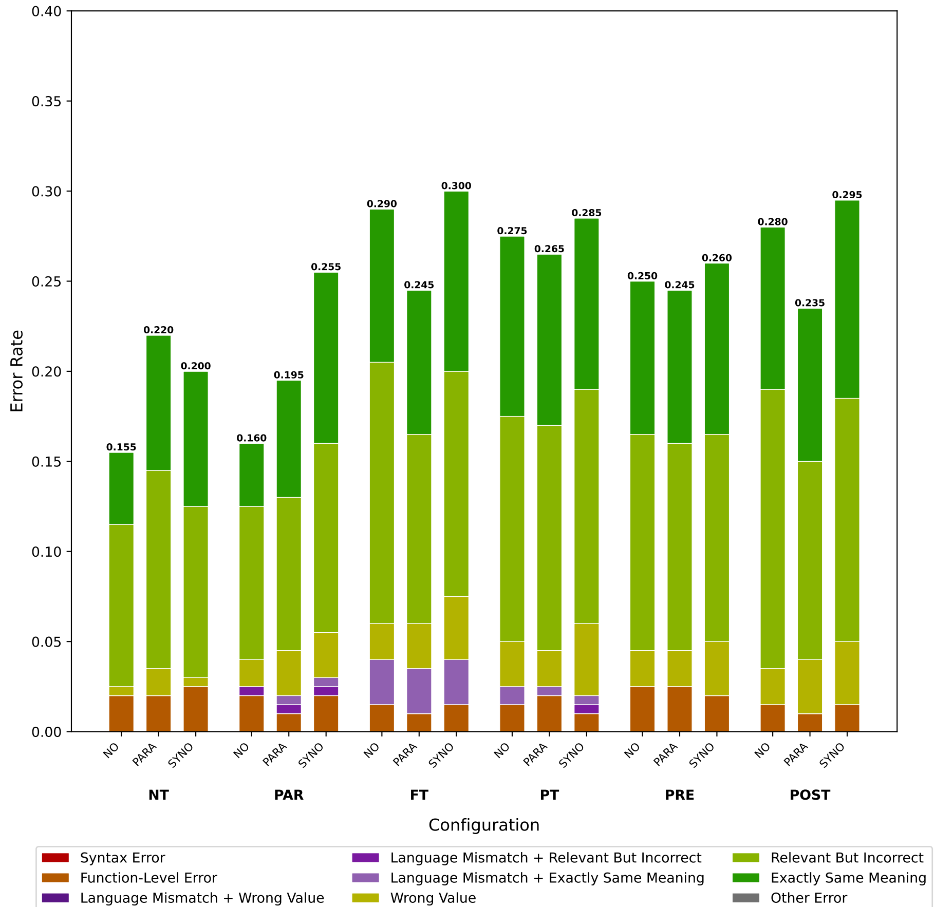
Tool Calling Errors of gpt-5-mini Under Hindi Queries
