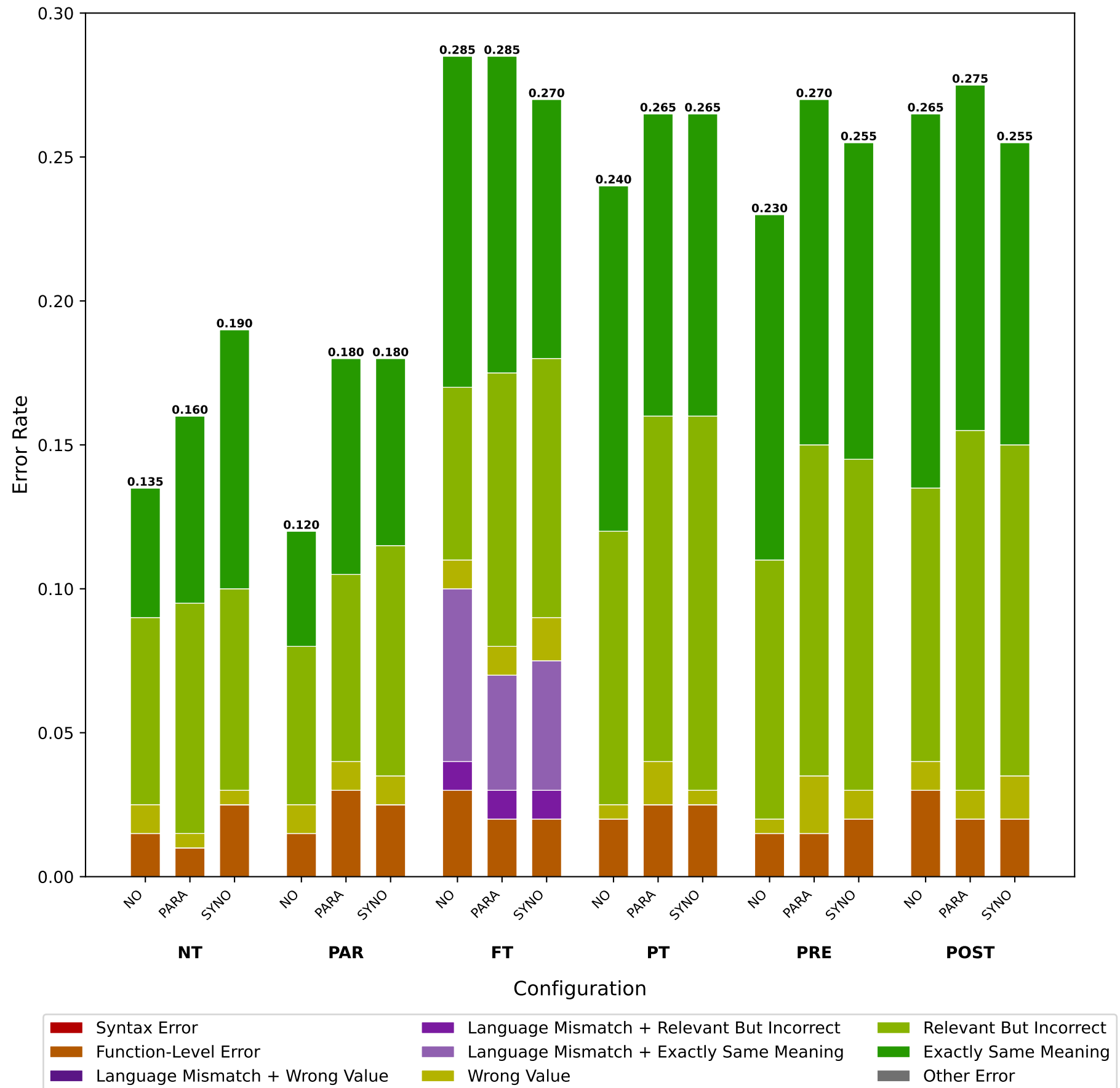
Tool Calling Errors of gpt-5 Under Chinese Queries
