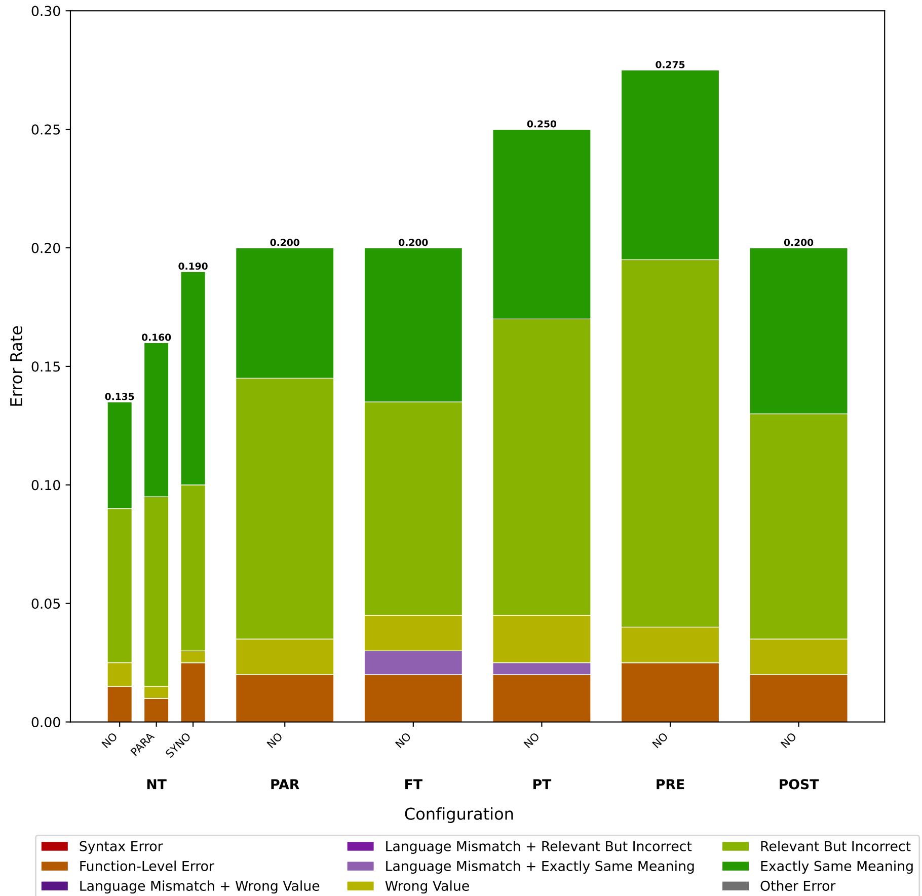
Tool Calling Errors of gpt-5 Under Igbo Queries
