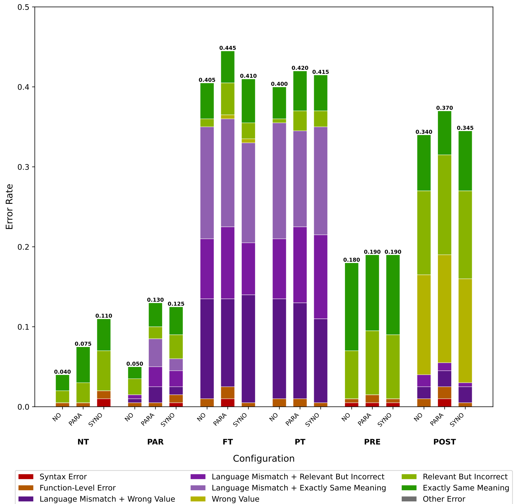
Tool Calling Errors of ibm-granite-granite-4.0-h-small Under Chinese Queries
