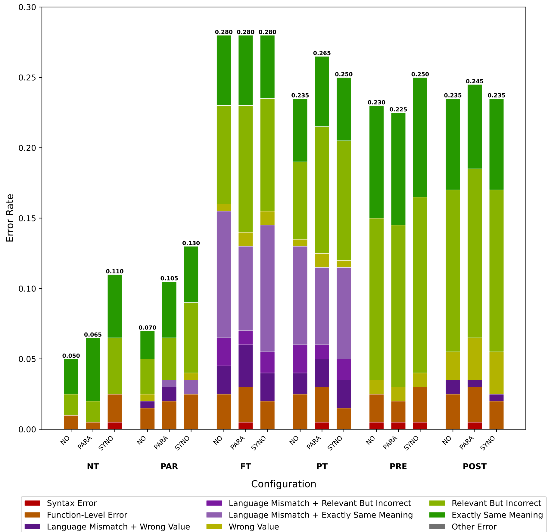
Tool Calling Errors of ibm-granite-granite-4.0-h-tiny Under Chinese Queries
