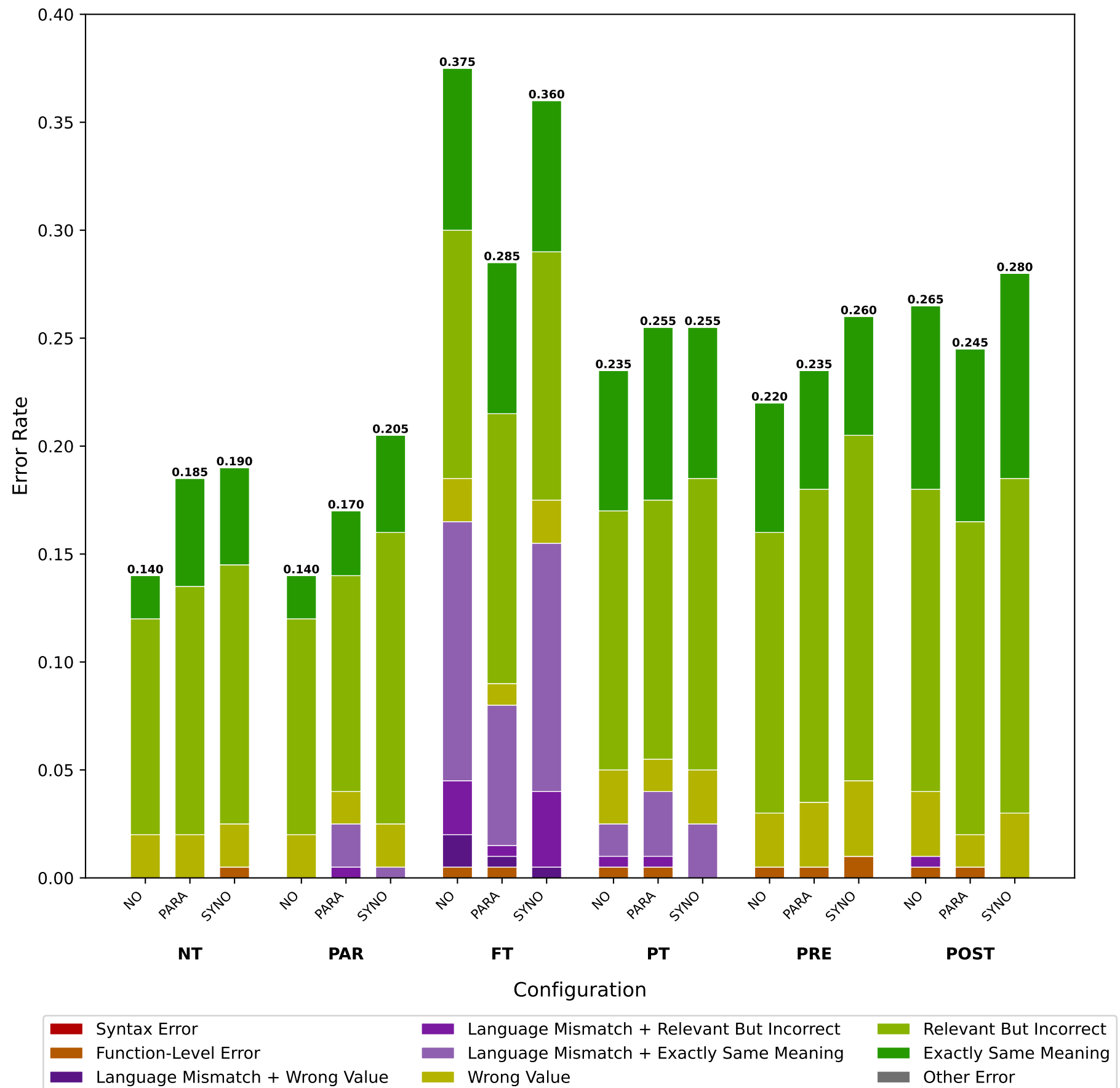
Tool Calling Errors of meta-llama-Llama-3.1-70B-Instruct Under Hindi Queries
