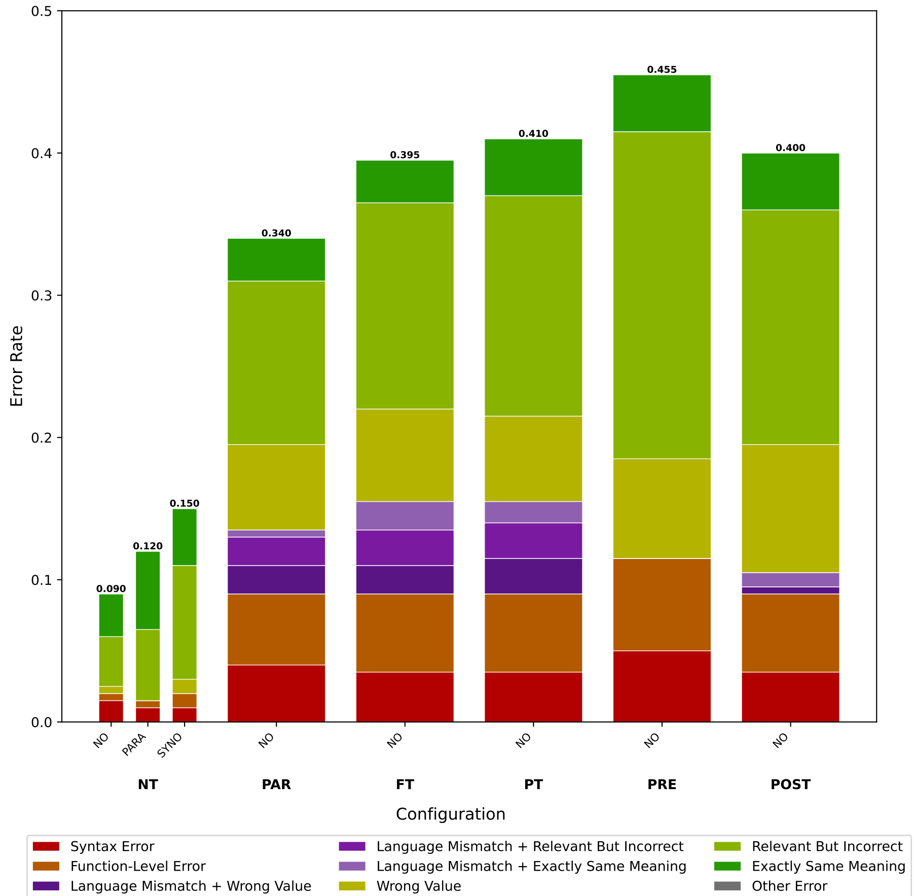
Tool Calling Errors of meta-llama-Llama-3.1-8B-Instruct Under Igbo Queries
