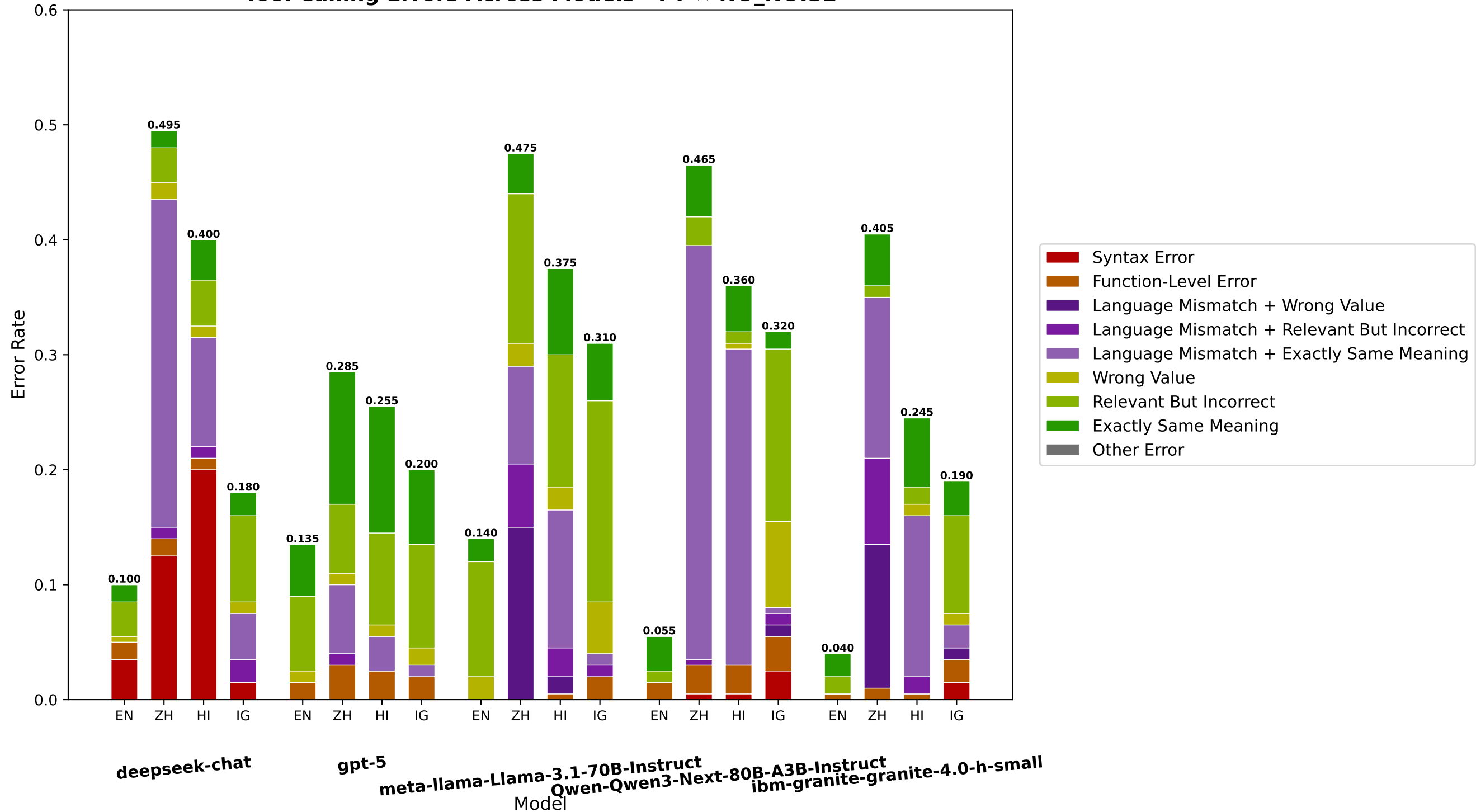
Tool Calling Errors Across Models - FT × NO_NOISE
