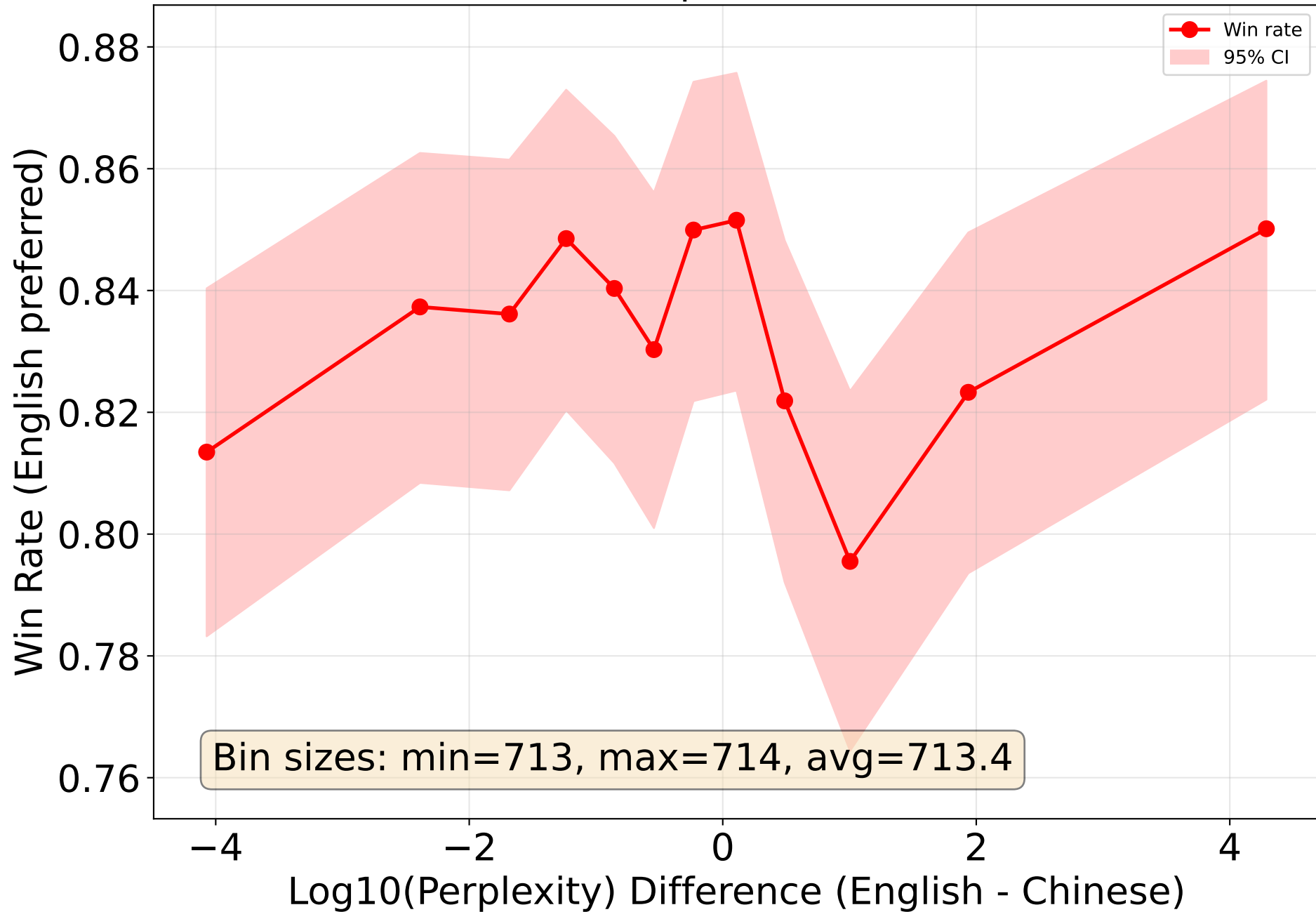
Win Rate vs. Perplexity Difference English incorrect answer vs. Chinese incorrect answer (n=8561 points, 12 bins)
