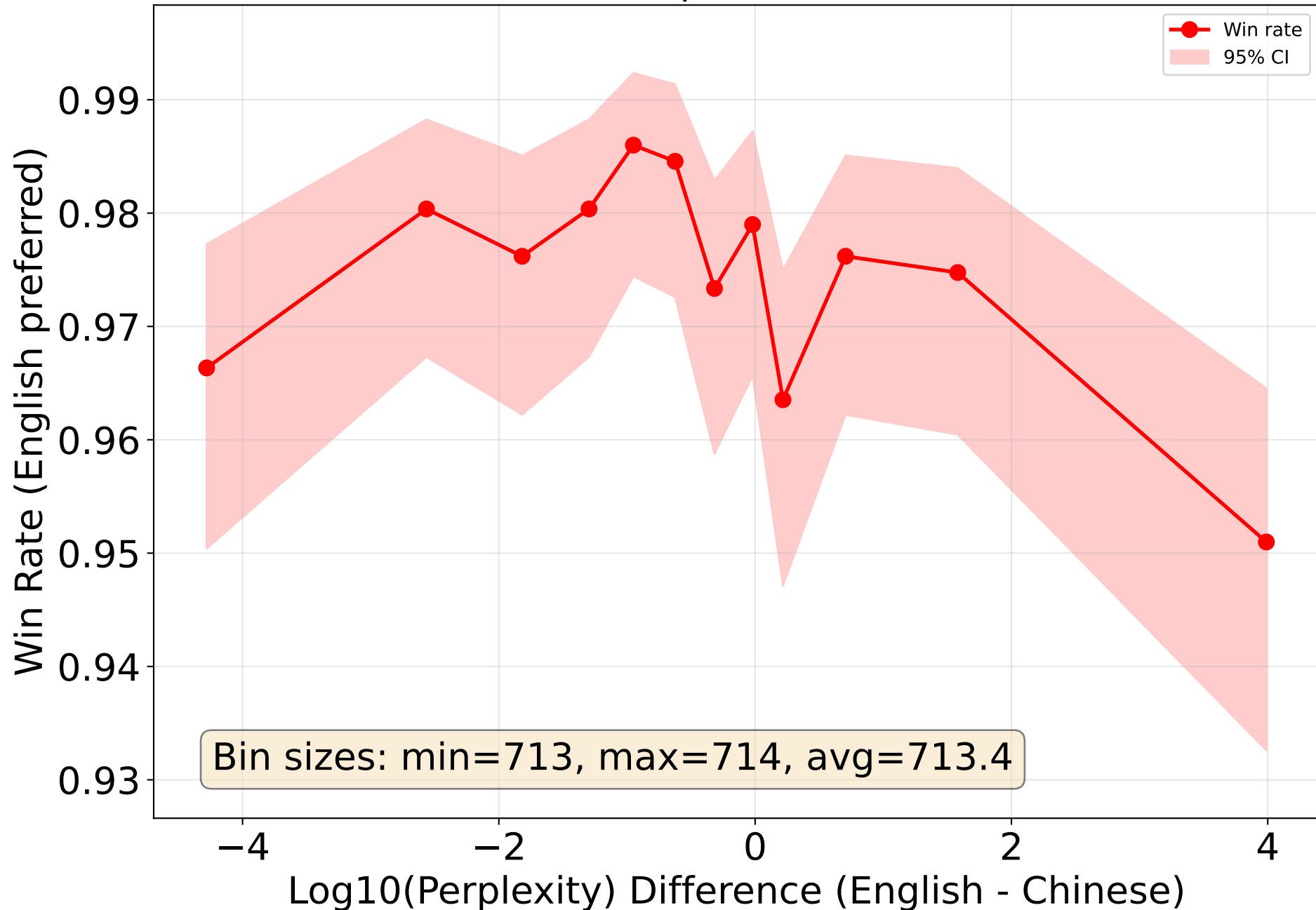
Win Rate vs. Perplexity Difference English correct answer vs. Chinese correct answer (n=8561 points, 12 bins)
