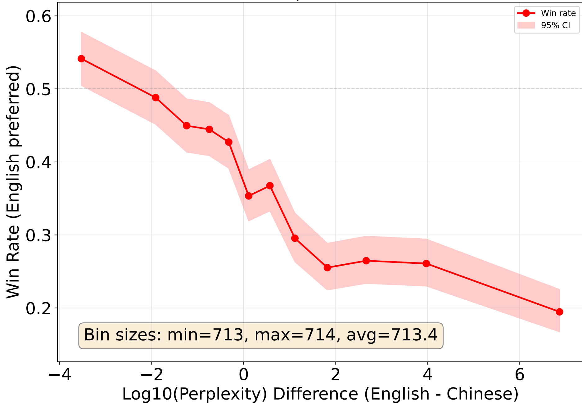
Win Rate vs. Perplexity Difference English incorrect answer vs. Chinese correct answer (n=8561 points, 12 bins)
