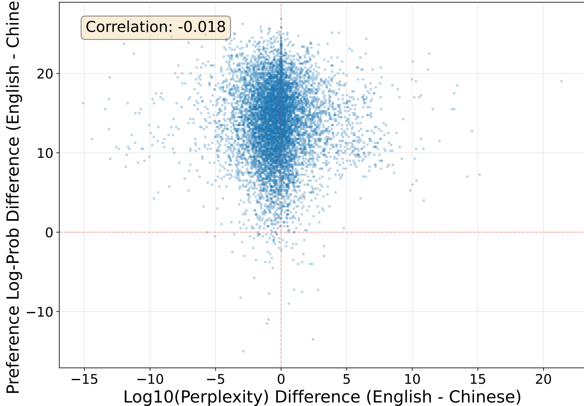
Preference Log-Prob Difference vs. Perplexity Difference English correct answer vs. Chinese correct answer (n=8561)
