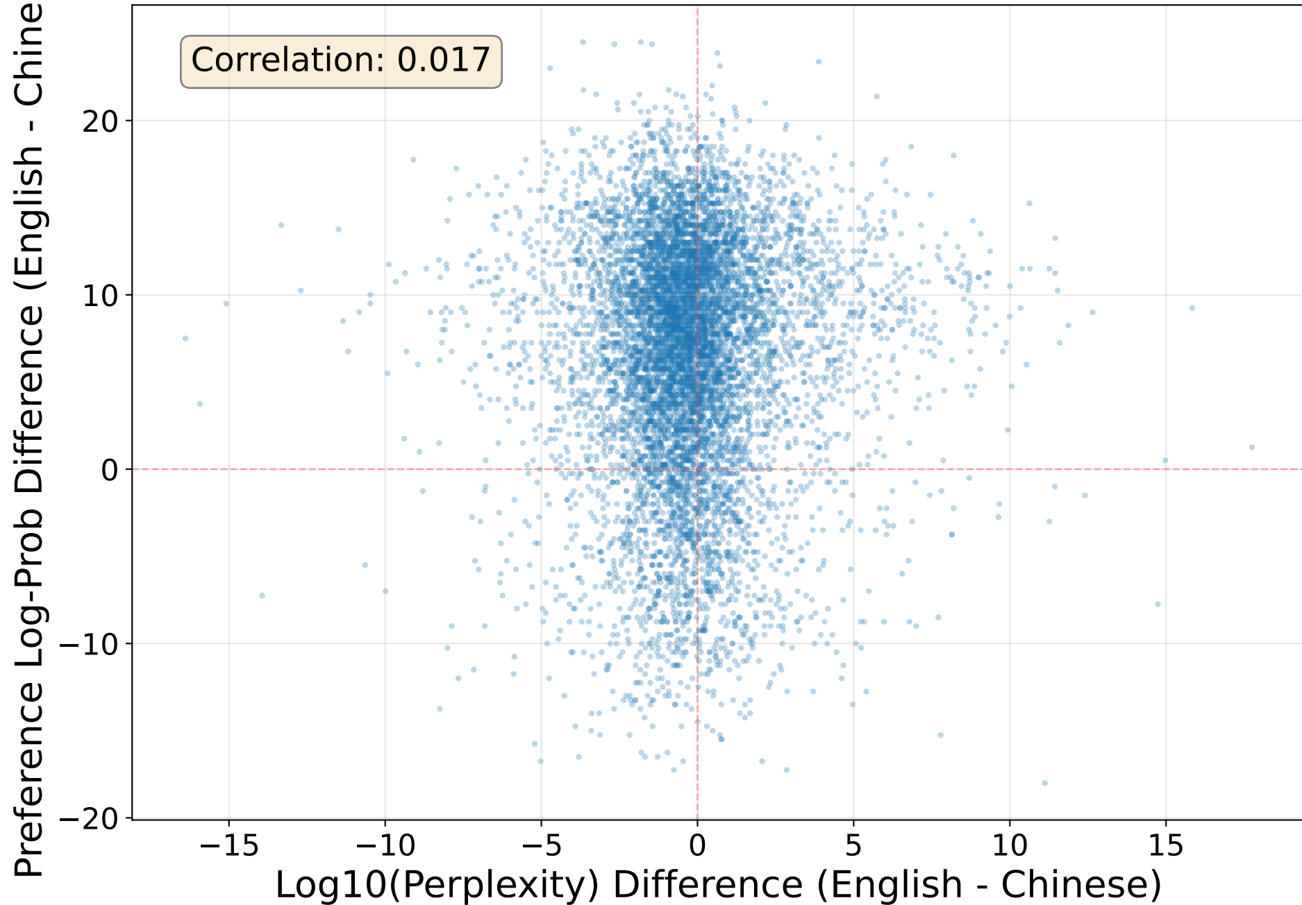
Preference Log-Prob Difference vs. Perplexity Difference English incorrect answer vs. Chinese incorrect answer (n=8561)
