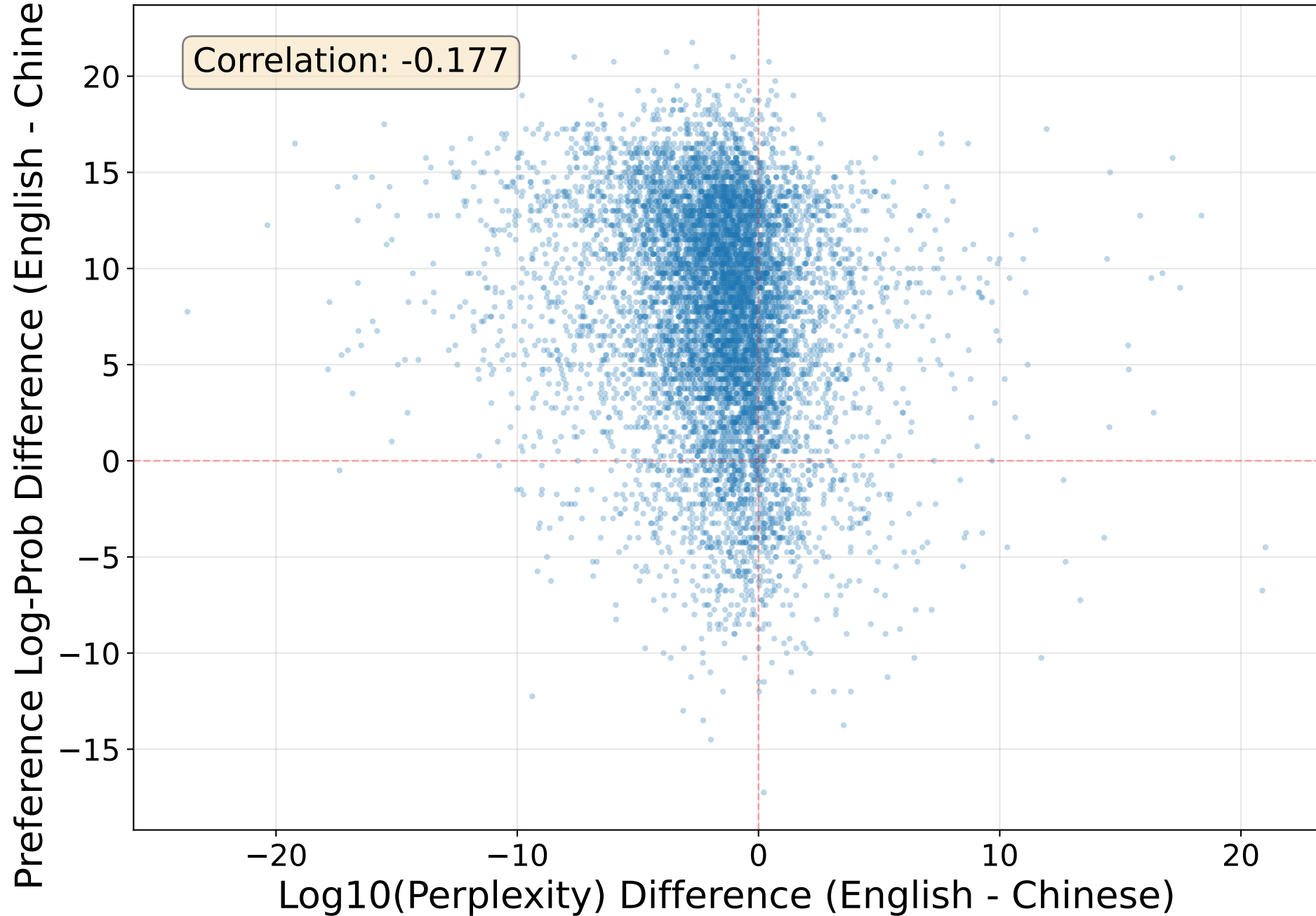
Preference Log-Prob Difference vs. Perplexity Difference English correct answer vs. Chinese incorrect answer (n=8561)
