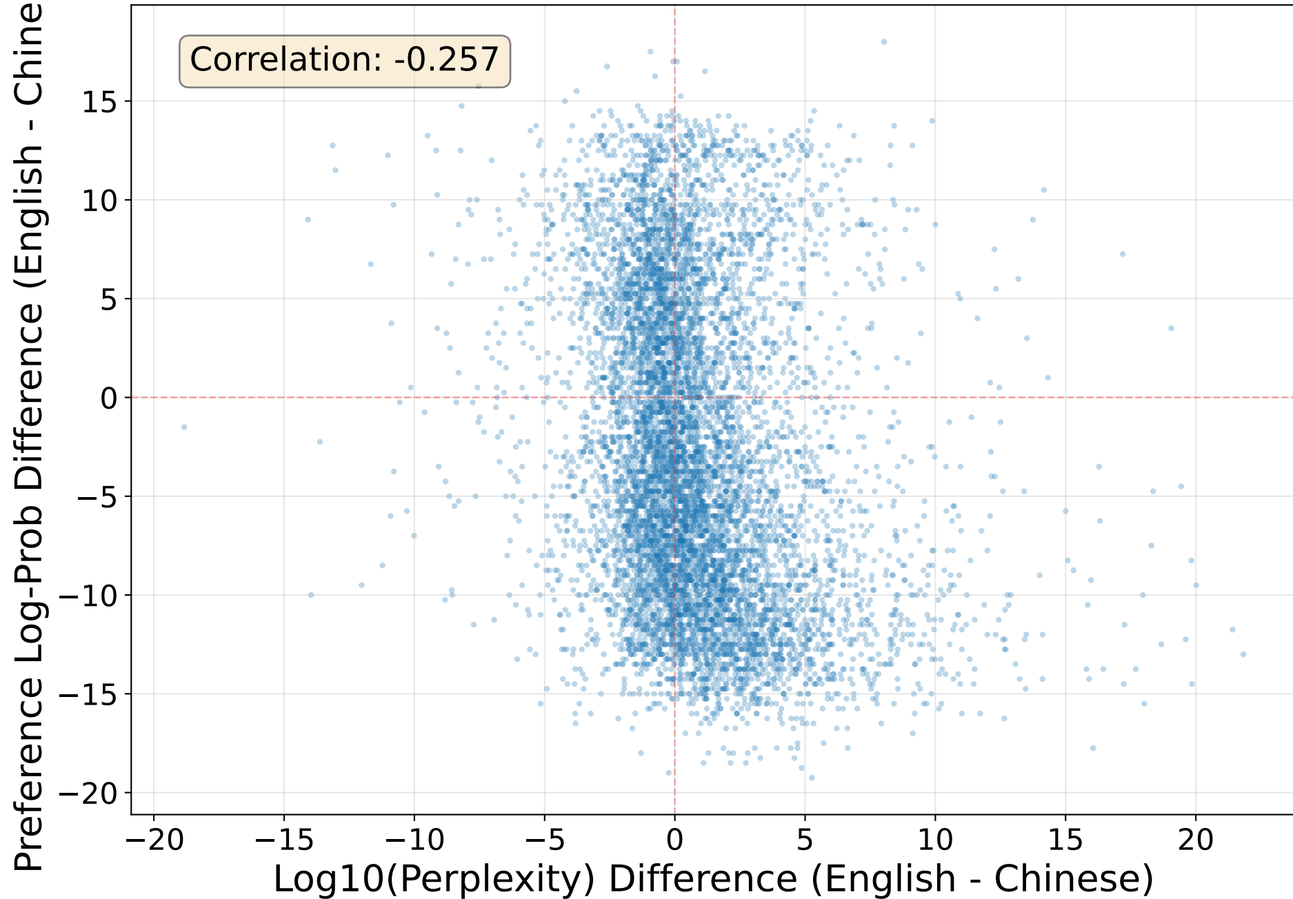
Preference Log-Prob Difference vs. Perplexity Difference English incorrect answer vs. Chinese correct answer (n=8561)
