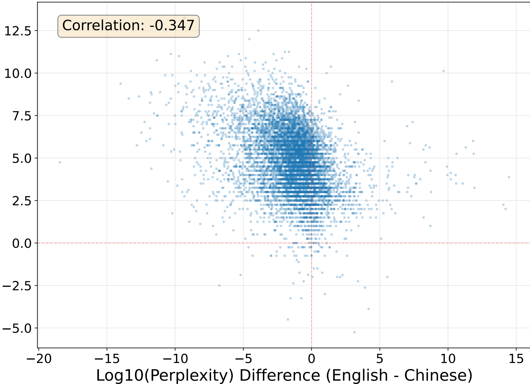
Preference Log-Prob Difference vs. Perplexity Difference English correct answer vs. Chinese incorrect answer (n=8561)
