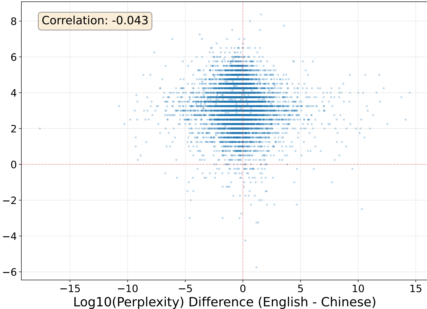
Preference Log-Prob Difference vs. Perplexity Difference English incorrect answer vs. Chinese incorrect answer (n=8561)
