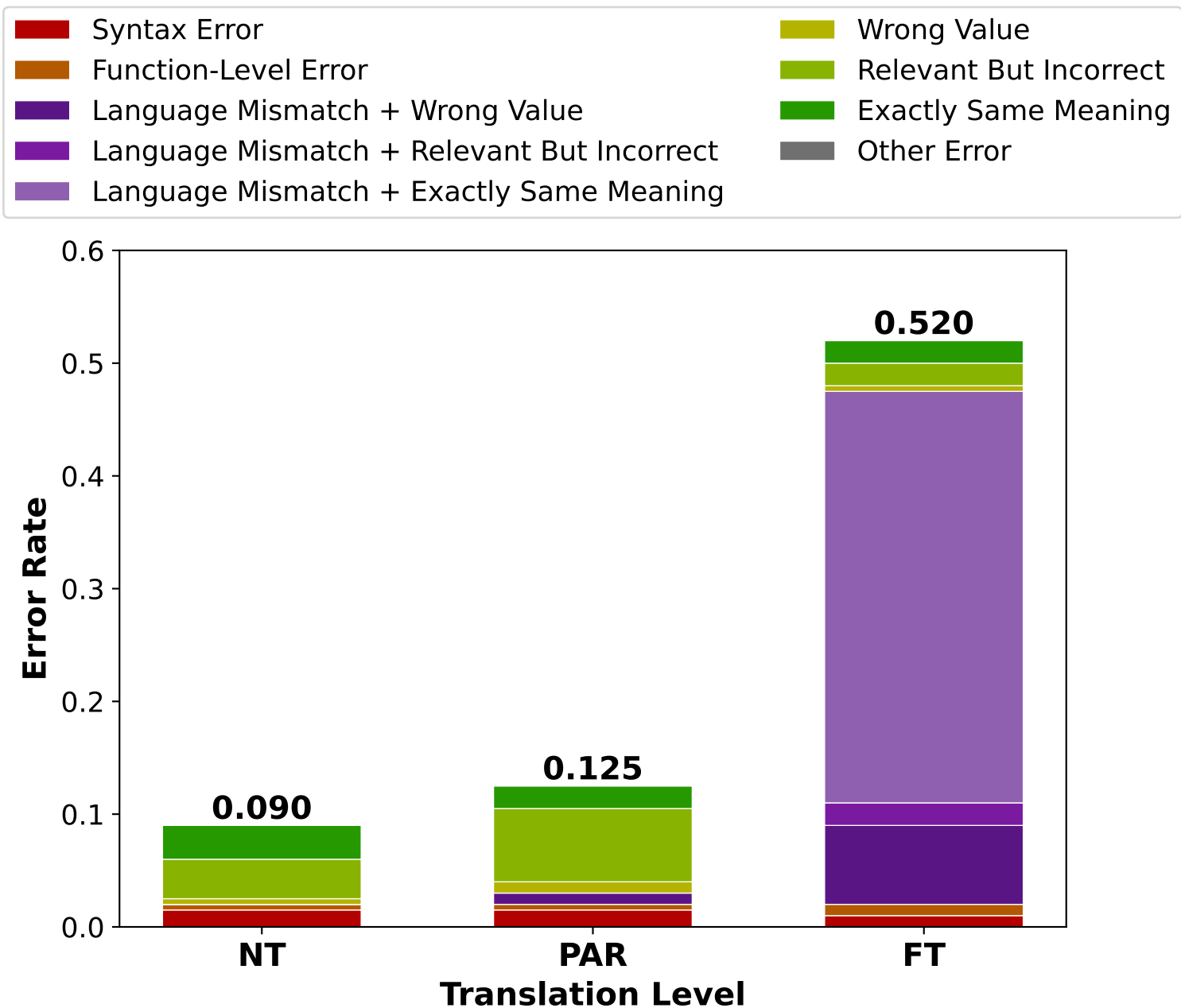
meta-llama-Llama-3.1-8B-Instruct's performance on Hindi datasets of different translation levels (no semantic perturbation added)
